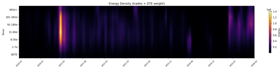
Figure 8: Energy density heatmap across time × tenor. The January 2021 squeeze is the only event to light up the entire tenor stack; during 2022-2023, energy persists at 181-365d even as shorter tenors go cold.
