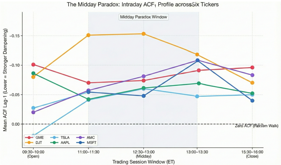
Figure 1: Intraday ACF 1 Profile showing how the Long Gamma Default builds throughout the trading session, peaking during the lowest-volume midday hours.
