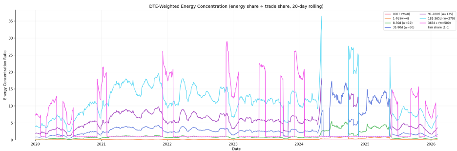
Figure 6: Energy concentration ratio over time. LEAPS (365d+) consistently operates at 10-30× its fair share; 181-365d stays at 8-15×. Short tenors (oDTE, 1-7d) are flat at 0.1-0.3×.
